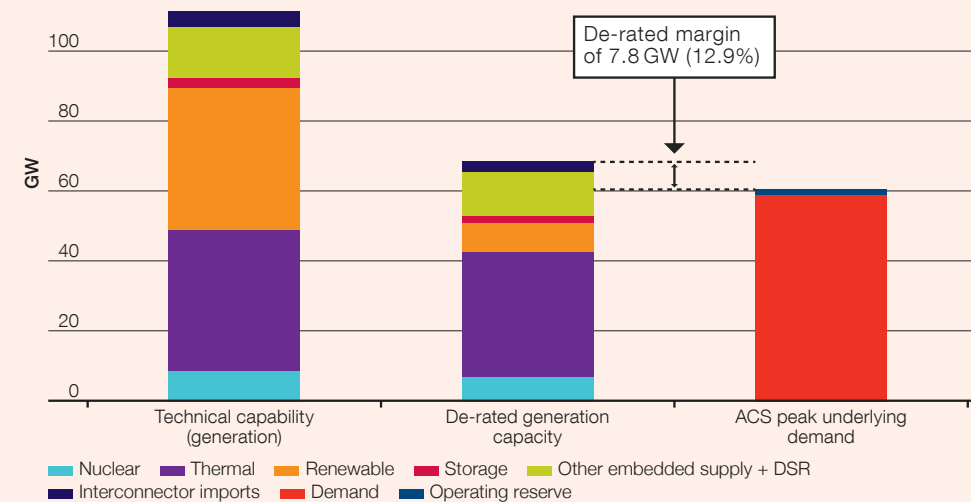
Figure 4.1 Supply margin in relation to generation capacity and demand
