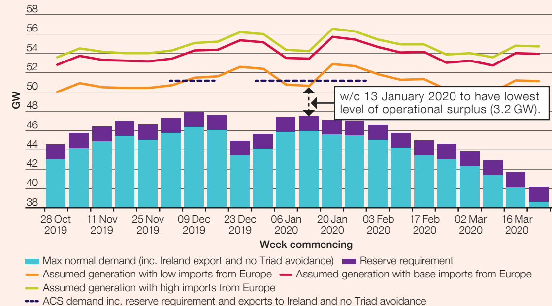
Figure 4.2 Week-by-week view of operational surplus for winter 2019/20
