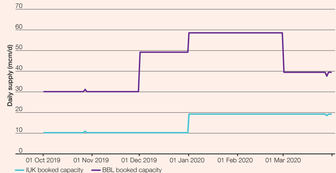
Figure 3.5 IUK and BBL booked capacity for winter 2019/20
