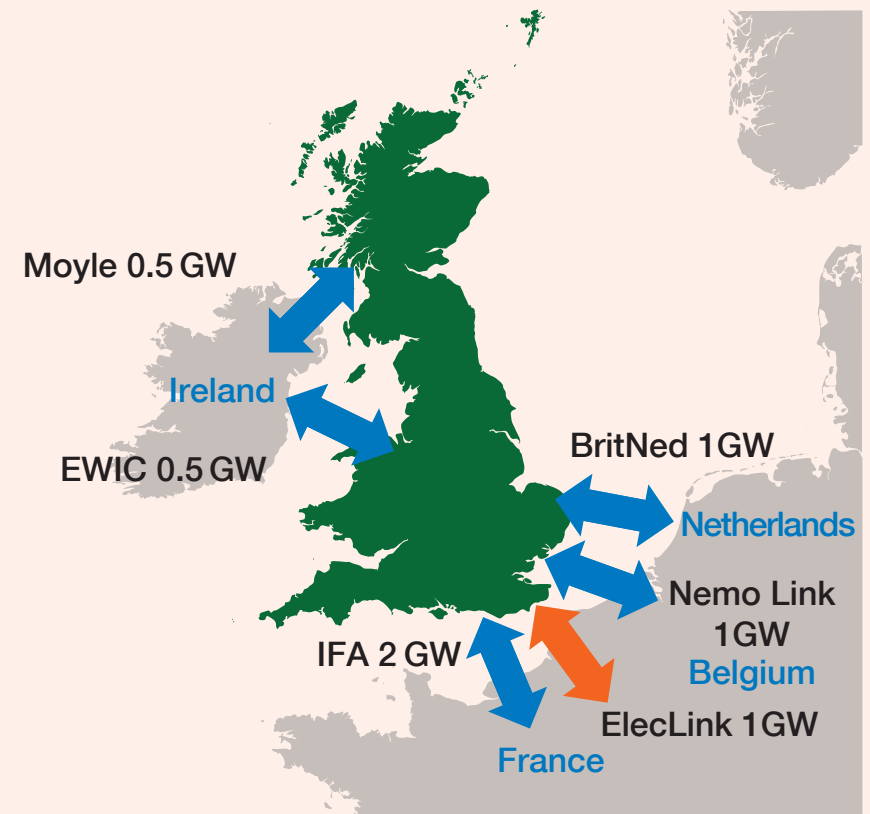
Figure 4.7 GB’s electricity interconnectors maximum physical capacity 5
