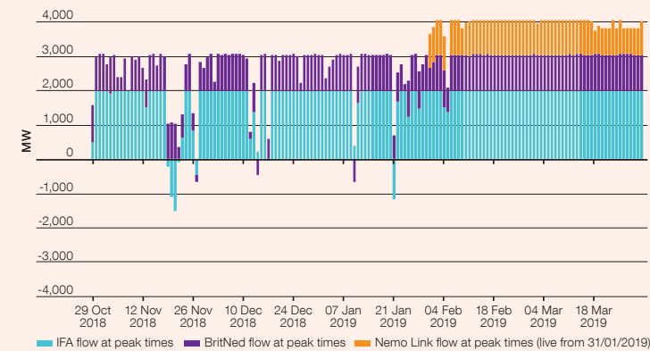
Figure 4.11 Proportion of import and export for continental interconnectors during winter 2018/19
