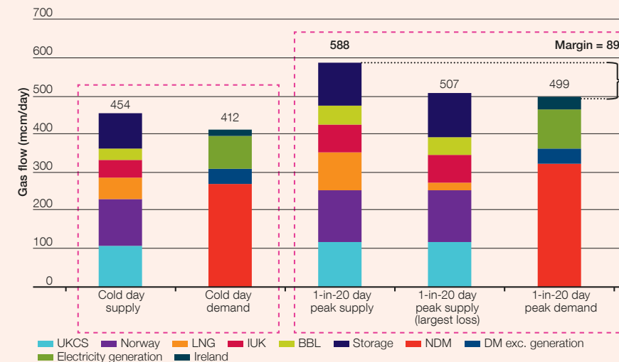
Figure 3.1 Supply and demand 1 on a cold day and a 1-in-20 peak day
