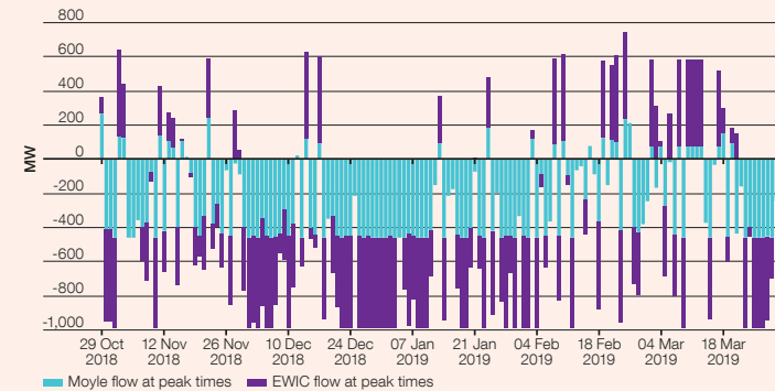
Figure 4.12 Daily peak time flows across the Irish interconnectors in winter 2018/19 (positive MW values mean imports into GB)
