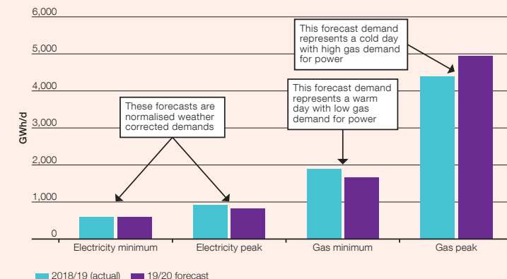
Figure 2.2 Minimum to peak day transmission level demands for gas and electricity (outturn from winter 2018/19 1 and forecast for winter 2019/20)
