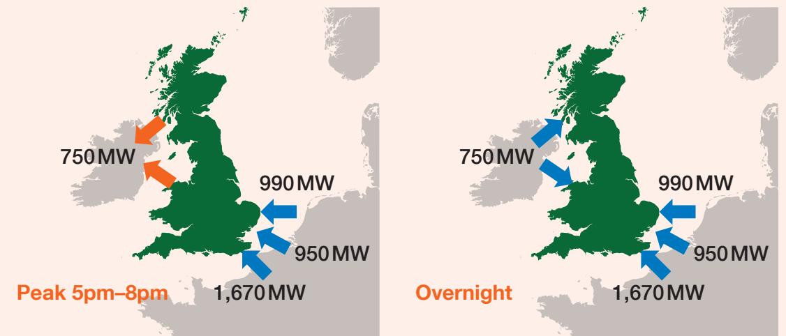
Figure 4.5 Forecast flows (high import scenario) on the interconnectors for winter 2019/20
