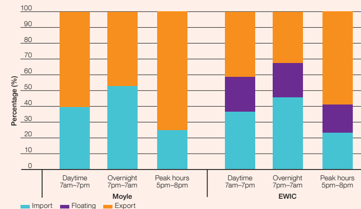
Figure 4.13 Proportion of import and export for Irish interconnectors during winter 2018/19
