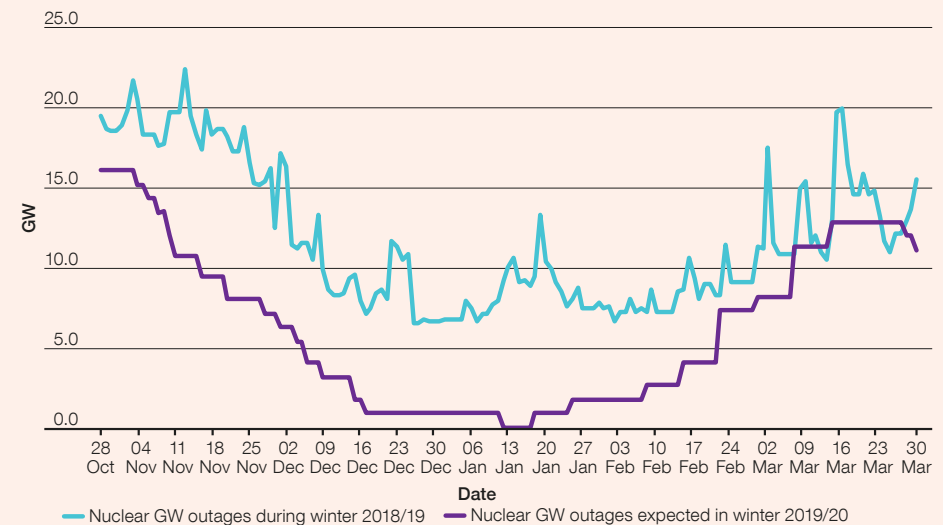
Figure 4.9 The impact on French nuclear capacity from planned outages in 2019/20 and last winter's actuals
