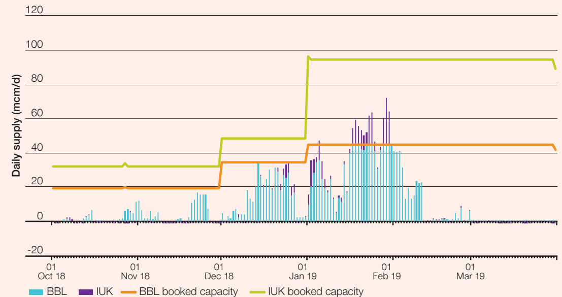
Interconnector flows and booked capacity for winter 2018/19
